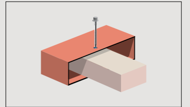
Wooden boards are screwed from the slots where the forklift forks are inserted. Two or three A-Frames are fixed by screwing the wooden boards, which have been passed through the Frames, to the outward-facing sides of the truck trailer. If there is no screw hole on the A-Frame, it is fixed with 5.5x90 DIN7504k, Hexagon drill-tip trapeze-panel screws with EPDM Rubber Washer.
