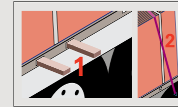
1- To support one or three A-Frames in a row, two wooden boards, which have at least 7x9 cm cross-sections and 240cm lengths, are used and placed in the forklift lifting slots.
